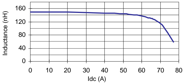
59PR72-221 Inductance vs. I dc @ 25°C
